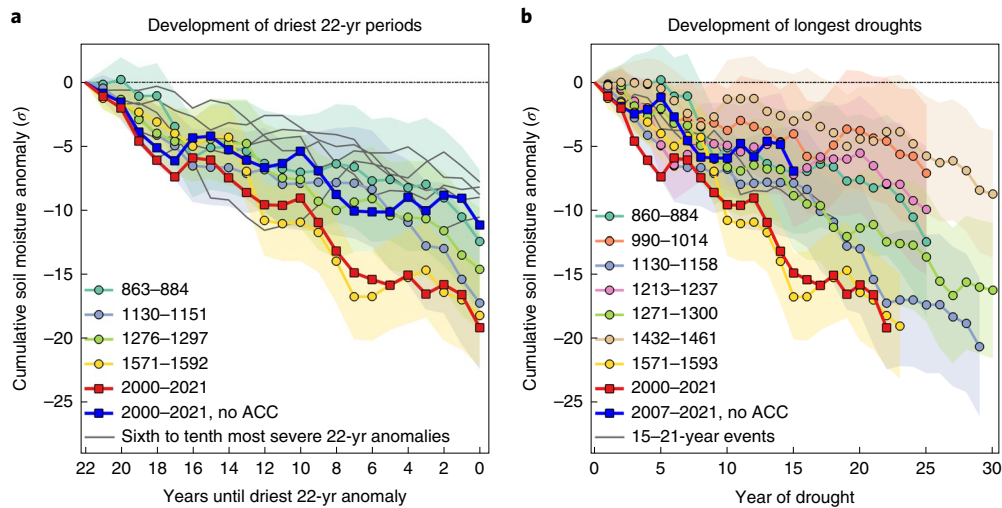
Fig. 2 | Trajectories of the most severe and longest extended droughts since 800 CE. a, b , Time series of cumulative SWNA soil moisture anomalies, in \sigma , during the development of the most negative 22-yr mean soil moisture anomalies ( a ) and from the beginning of all drought events \geq 15 yr long ( b ). Blue line, development of the 2000s drought after removing CMIP6 multimodel mean climate trends (no ACC) from the observed trajectory of the 2000s drought (red line). In b , each drought period ends in its final year (based on our definition of an extended drought event, described in Methods, the longest megadroughts lasted 30 yr). Note: the blue ACC line is shorter than the red observed line in b because the drought would not have started until 2007 in the absence of ACC contributions. Shading, 95% CI for the reconstructed droughts.
